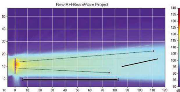
Beamware display of an Iconyx IC8 array's dual beam output.
