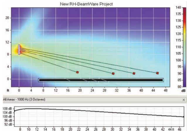
Beamware display showing the multi-beam capabilities of the IC8 Iconyx array.
