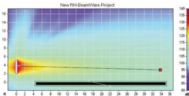
Beamware display of an Iconyx IC8 array's precisely controlled output
